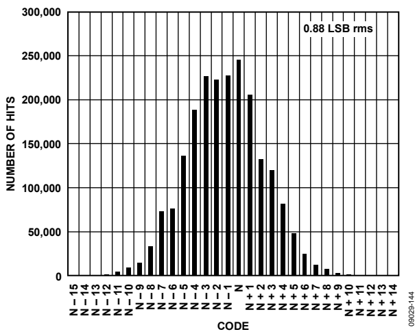
Figure 44. Input-Referred Noise Histogram, 2.5 V p-p FS, AD9467-250
