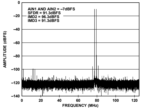
Figure 31. Two-Tone FFT with f_{IN1} = 170 MHz and f_{IN2} = 172 MHz, 2.5 V p-p FS, AD9467-250
