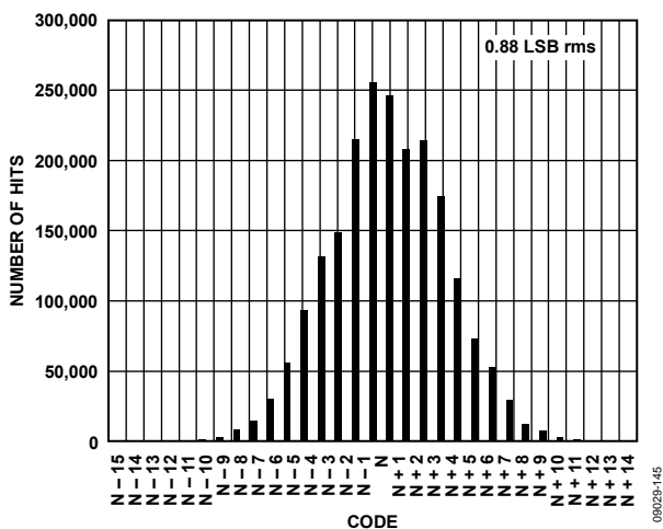
Figure 45. Input-Referred Noise Histogram, 2.5 V p-p FS, AD9467-200
