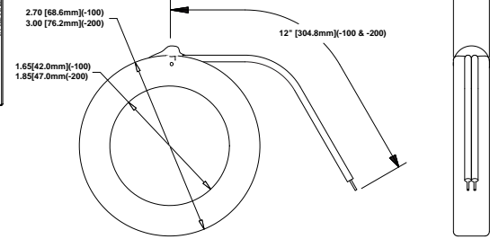
Remote Current Transformers CRGFS - Series
