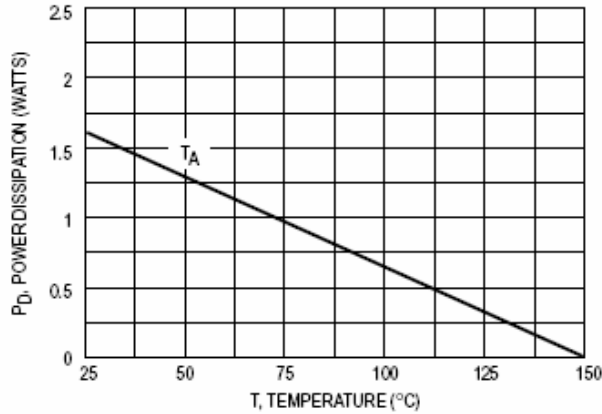
Figure 1. Power Derating
