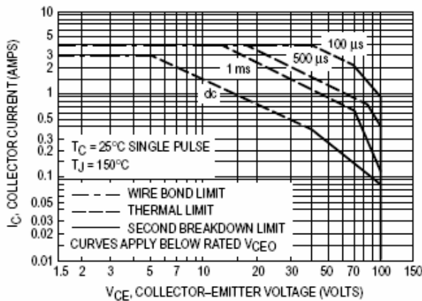
Figure 10. Active Region Safe Operating Area
