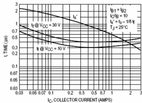
Figure 6. Turn-Off Time
