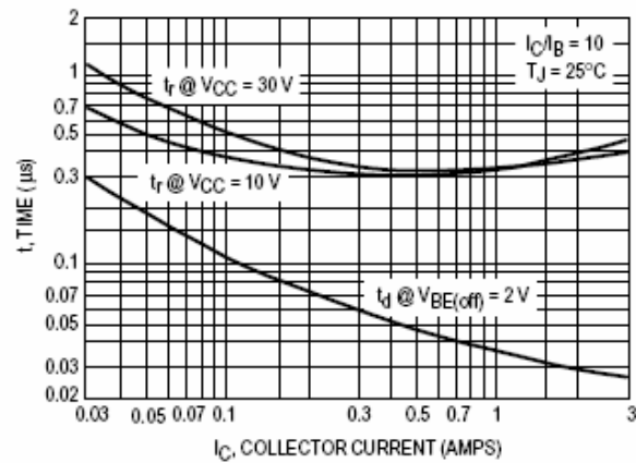
Figure 4. Turn-On Time
