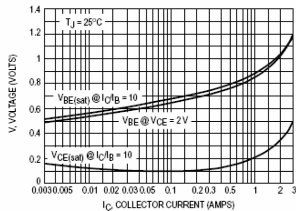
Figure 5. "On" Voltages
