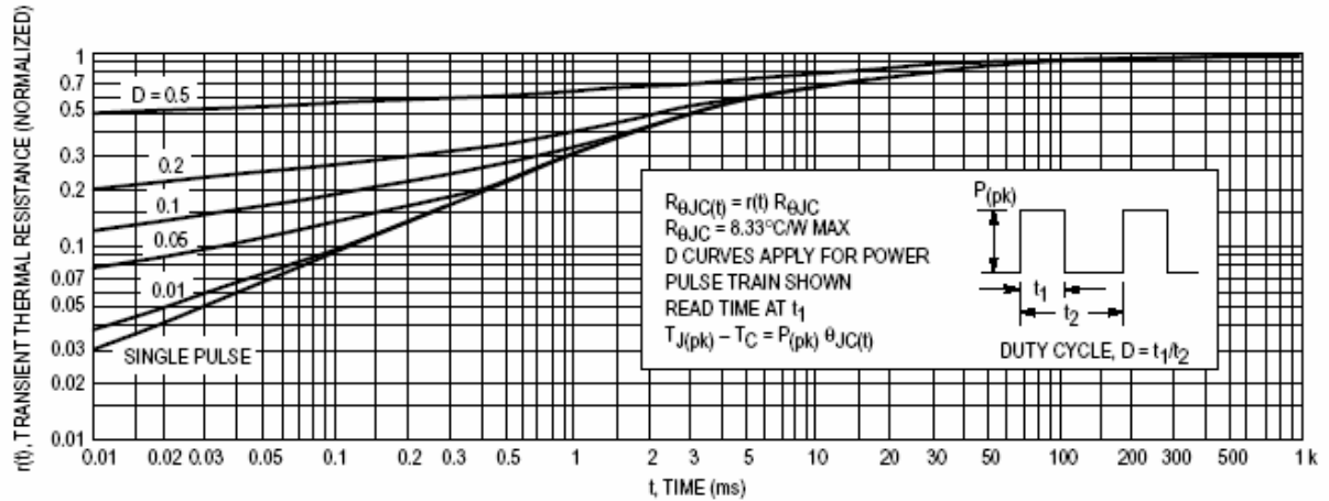
Figure 9. Thermal Response
