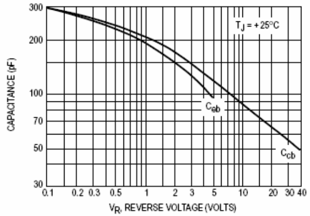
Figure 8. Capacitance
