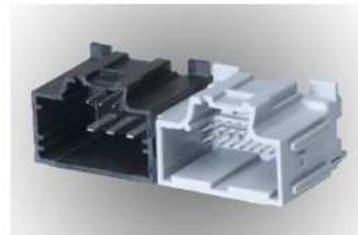
30-Circuit Ganged Vertical Header - With Power-Pocket Option
