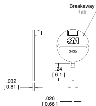
3435-0 Keying Plug
