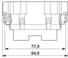
Male insert
