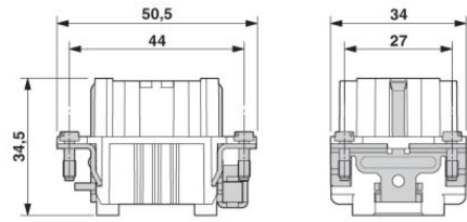
Female insert
