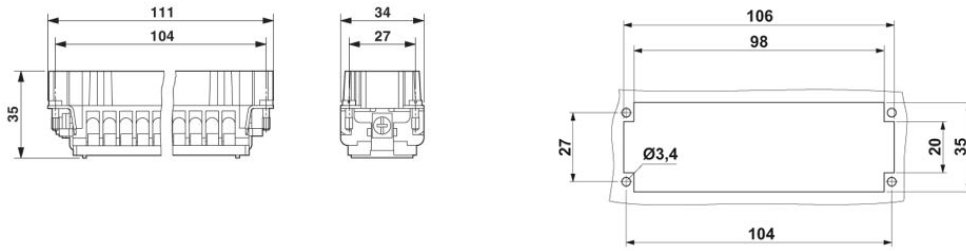
Mounting cut-out
