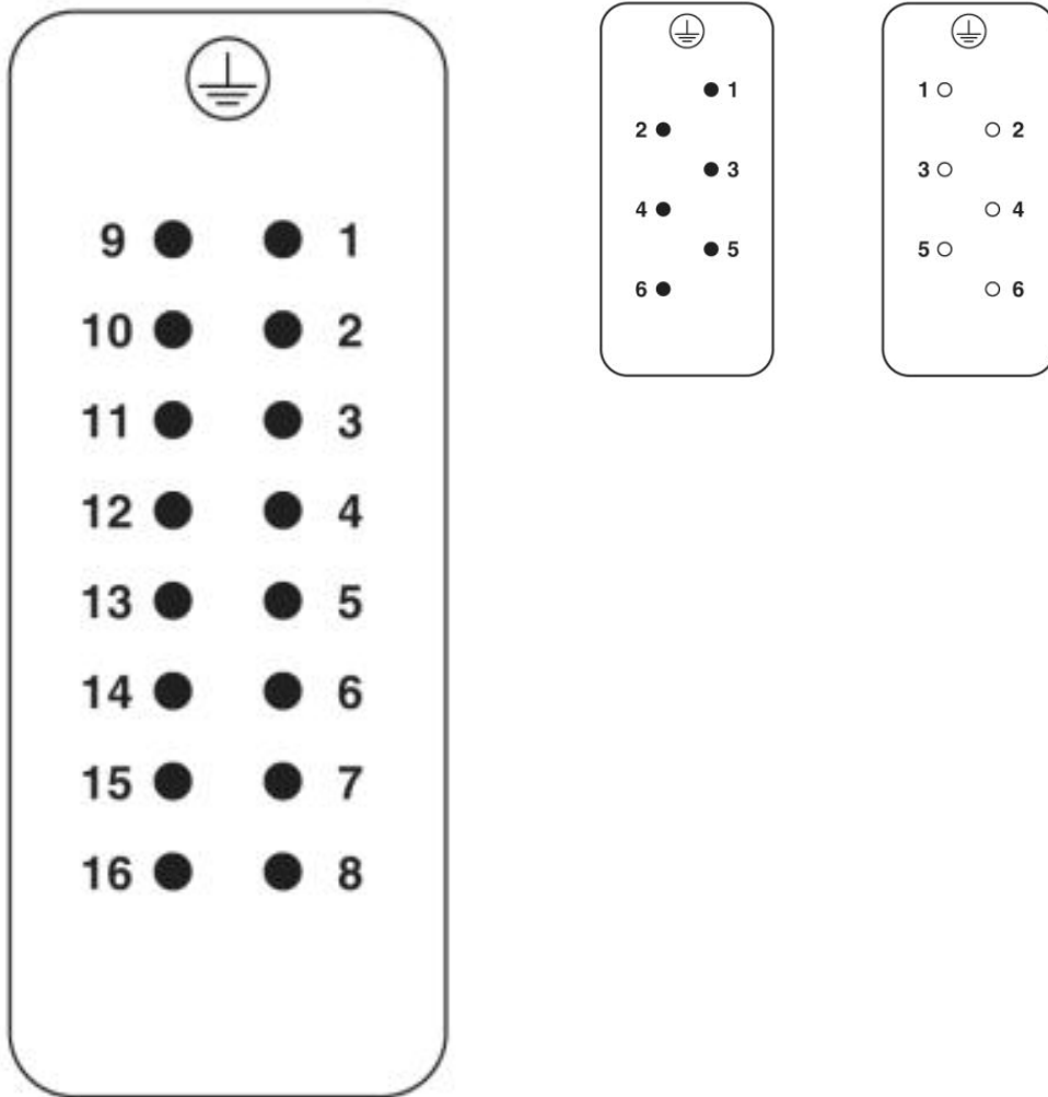
Connector pin assignment, connection side
