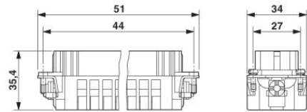
Female insert
