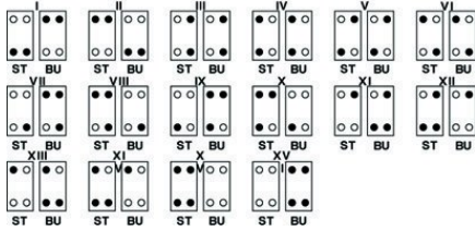
Coding for housings with one contact insert
