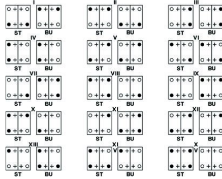
Coding for housings with two contact inserts
