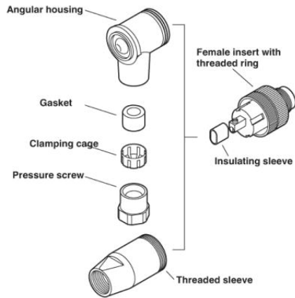
Male/Female M12
