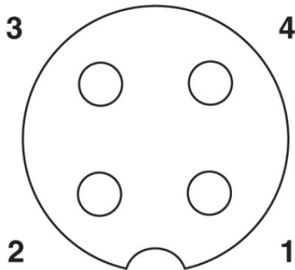
Male/Female M12
