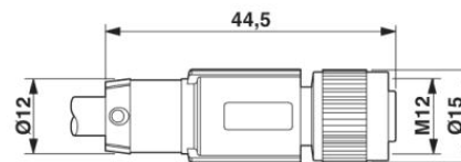
M12 x 1 female connector, straight
