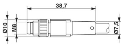
M8 x 1 male connector, straight version
