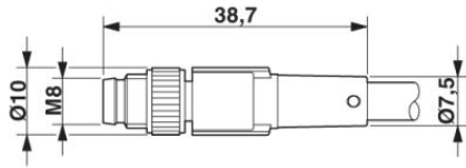
M8 x 1 male connector, straight version
