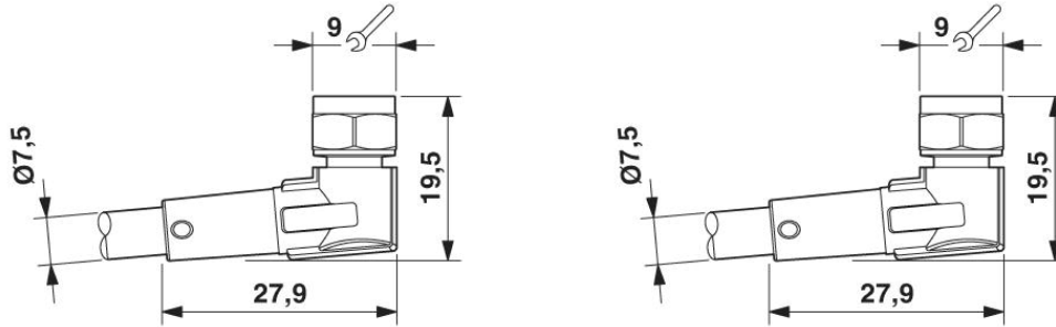
Socket M8 x 1, angled
