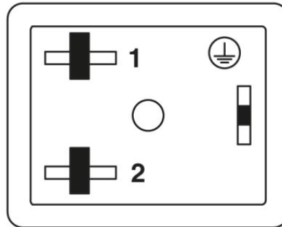
Valve connector pin assignment, type BI
