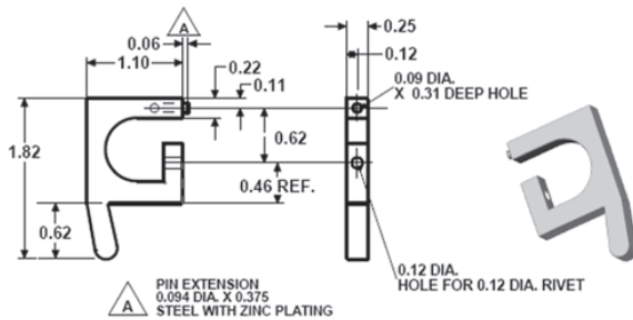
EFP204A66F - 2" EFP Modules with HA11 handle
