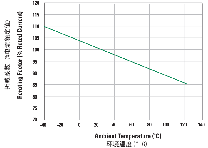
ATOF™ 保险丝温度折减曲线 ATOF™ Fuse Temperature Derating Curve
