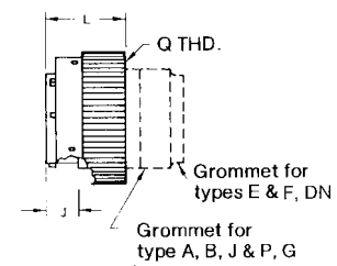
Crimp KPSE06/MS3126
