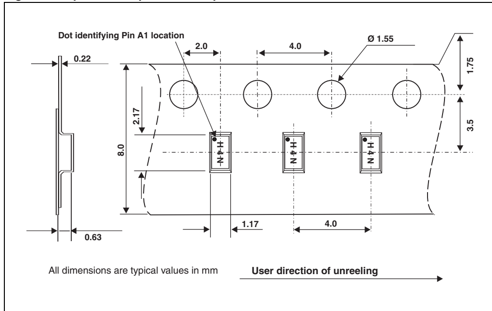
Figure 11. \mu QFN-8L tape and reel specification
