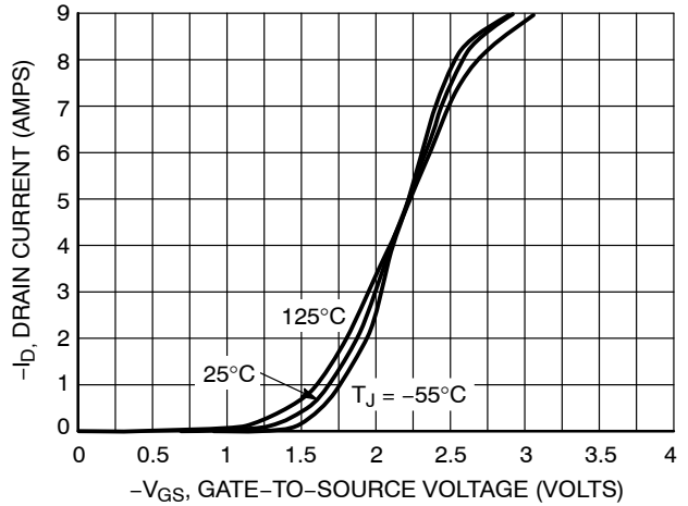
Figure 19. Transfer Characteristics
