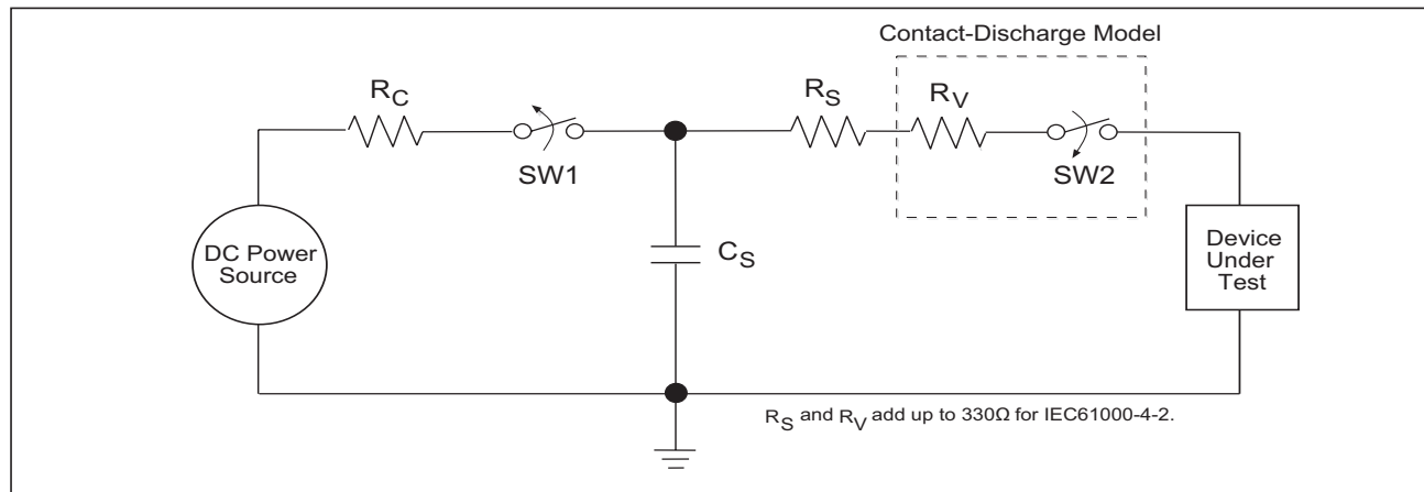
Figure 15. ESD Test Circuit for IEC61000-4-2
