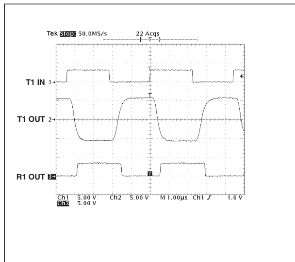
Figure 8. Loopback Test results at 460kbps
