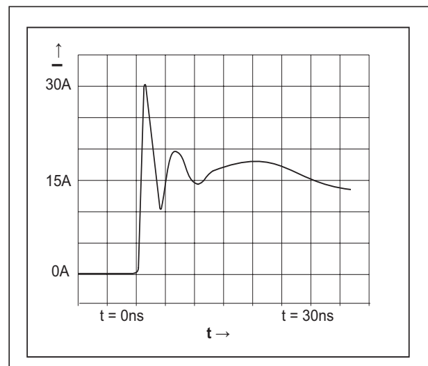
Figure 16. ESD Test Waveform for IEC61000-4-2
