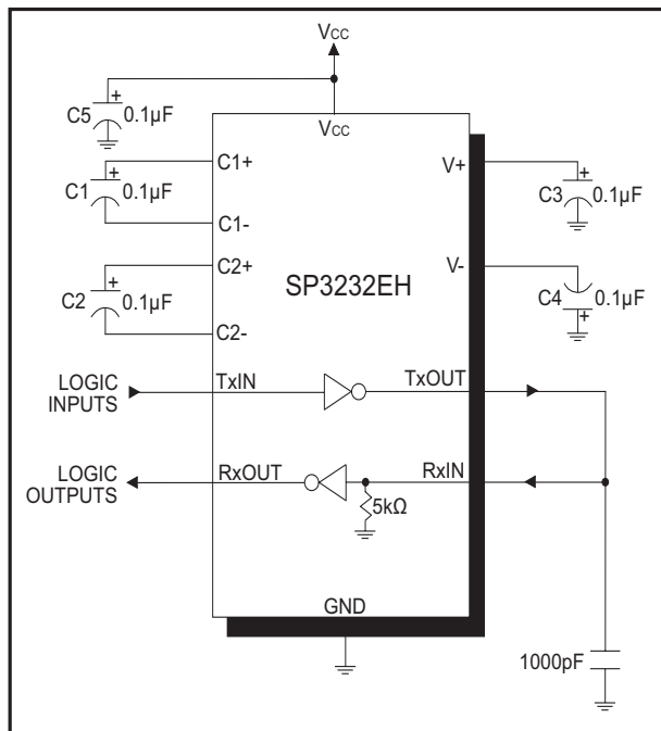
Figure 6. SP3232EH Driver Loopback Test Circuit
