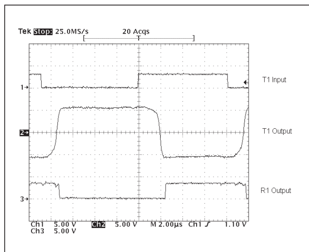
Figure 7. Loopback Test results at 120kbps
