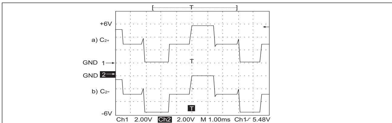
Figure 11. Charge Pump Waveforms
