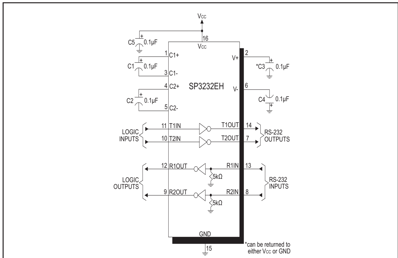
Figure 5. SP3232EH Typical Operating Circuit
