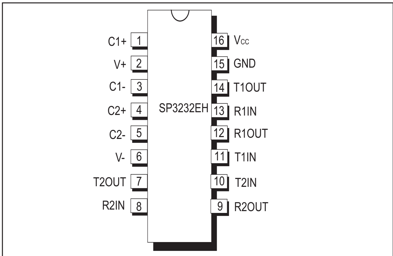
Figure 4. Pinout Configuration for the SP3232EH
