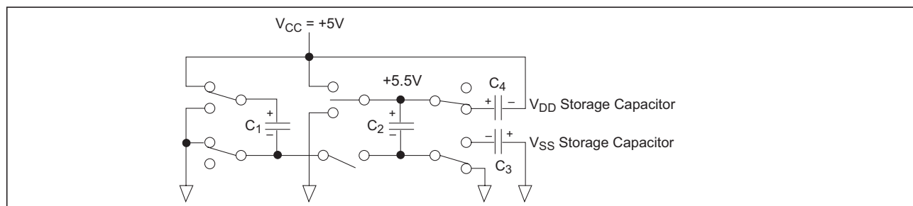
Figure 13. Charge Pump — Phase 4
