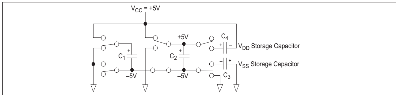
Figure 9. Charge Pump — Phase 1
