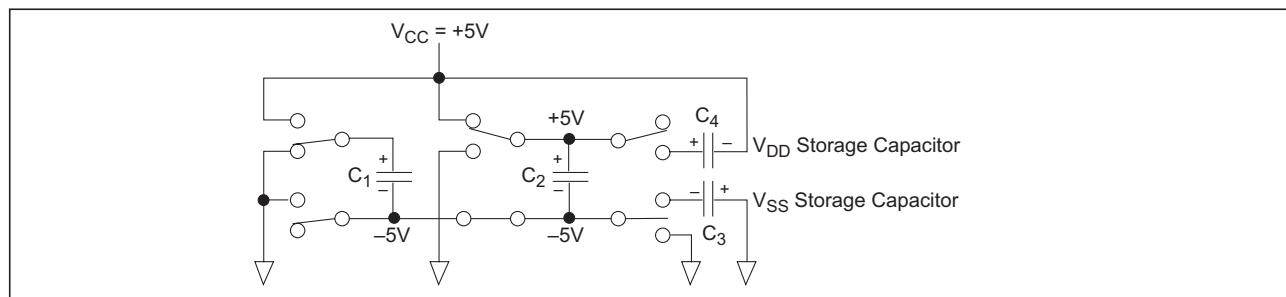
Figure 12. Charge Pump — Phase 3
