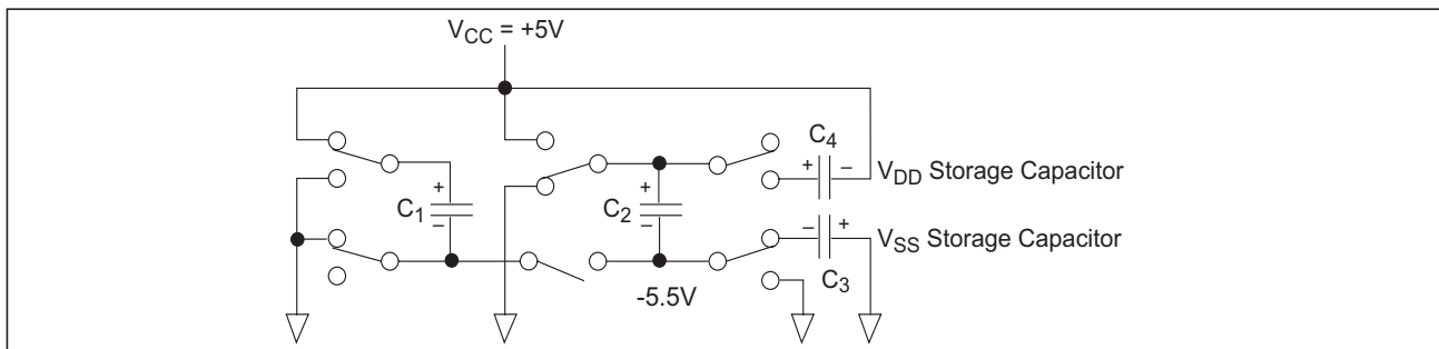
Figure 10. Charge Pump — Phase 2
