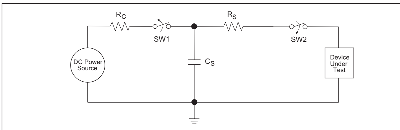
Figure 14. ESD Test Circuit for Human Body Model
