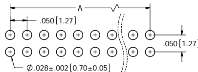
RECOMMENDED PCB HOLE LAYOUT
