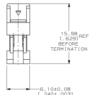
DETAIL Z SCALE 10:1 TYPICAL
