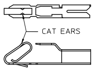
CAT EAR TERMINAL OPTION
