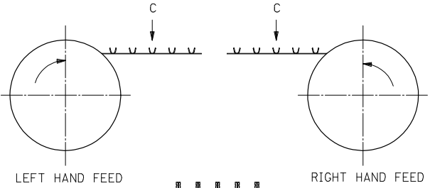
VIEW C
