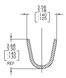
SECTION B-B SCALE 10:1
