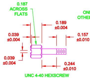
UNC 4-40 HEXSCREW
