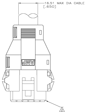
ASSEMBLED VIEW
