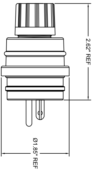
FACE VIEW OF PLUG
