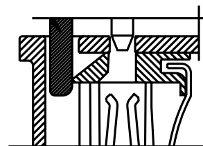
Shutter operation: shutters opened by plug insertion
