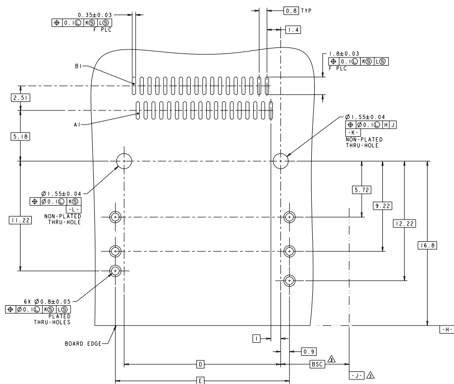
RECOMMENDED PCB LAYOUT SCALE 10:1
