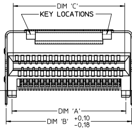
36 CIRCUIT RETENTION FIT SHELL OPTION SHOWN
