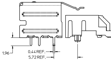
SMT SHELL OPTION
