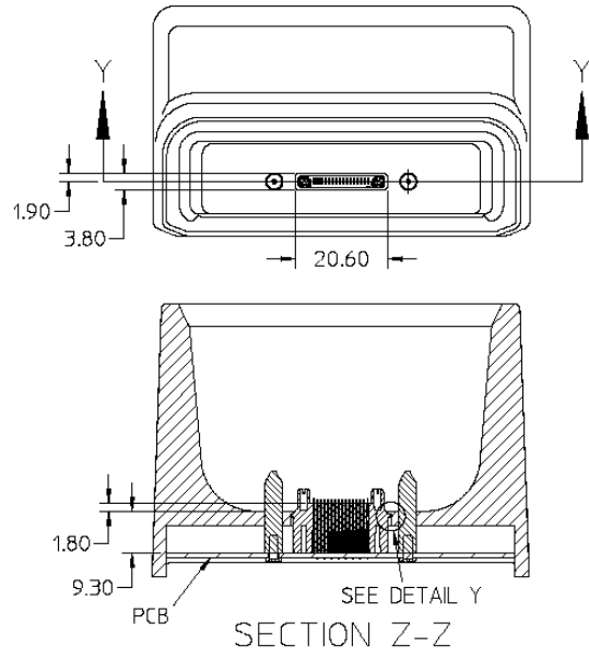
Figure 17. Cradle Detail (45593) (units: mm)
