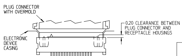
RECOMMENDATIONS FOR CONFIGURATION OF MATED CONNECTORS
