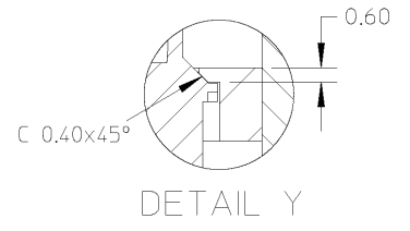
Figure 18. Detail from Fig. 17. (units: mm)
