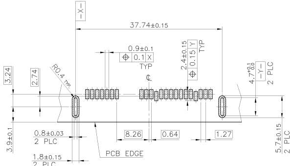
RECOMMENDED P.C.B. LAYOUT (THICKNESS=1.2)
