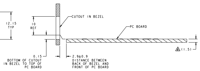
SECTION F-F RECOMMENDED BEZEL CONFIGURATION
