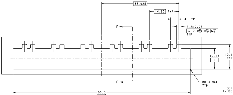
RECOMMENDED BEZEL CUTOUT
