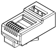
PLUG HOUSING SCALE 2.5
