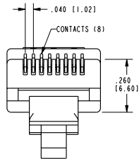
PLUG HOUSING SCALE 2.5
