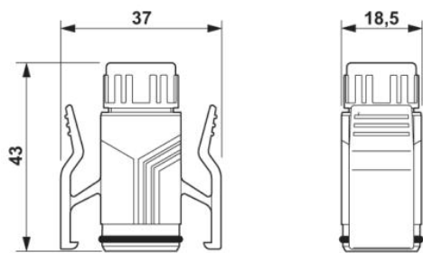
RJ45 sleeve housing IP67
