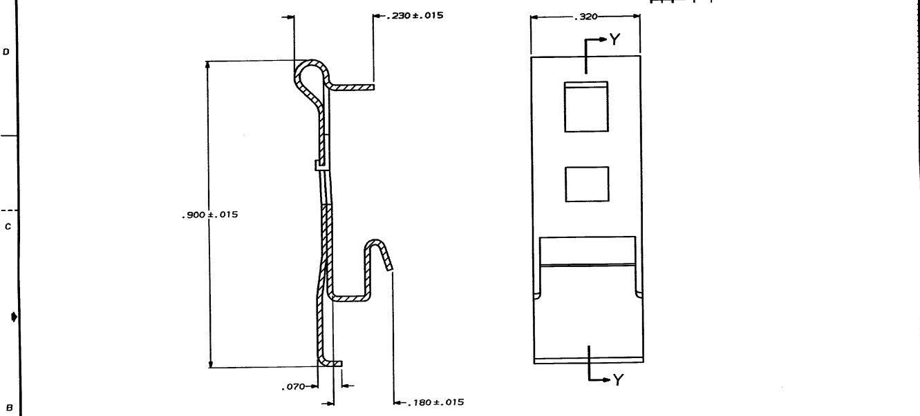
SECTION Y-Y
