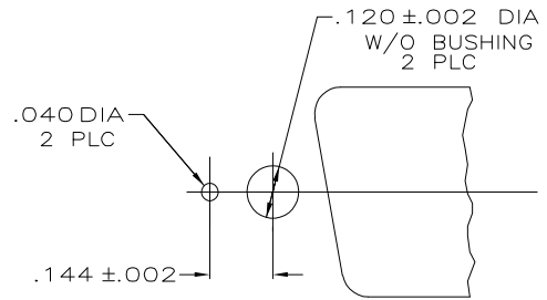
PANEL CUTOUT DETAIL NTS
