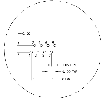
Pin Designations
