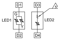
LED CONFIGURATION FOR 5-6605758-4 ONLY
