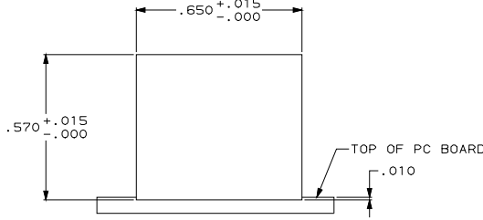
SUGGESTED PANEL CUTOUT SCALE 4:1
