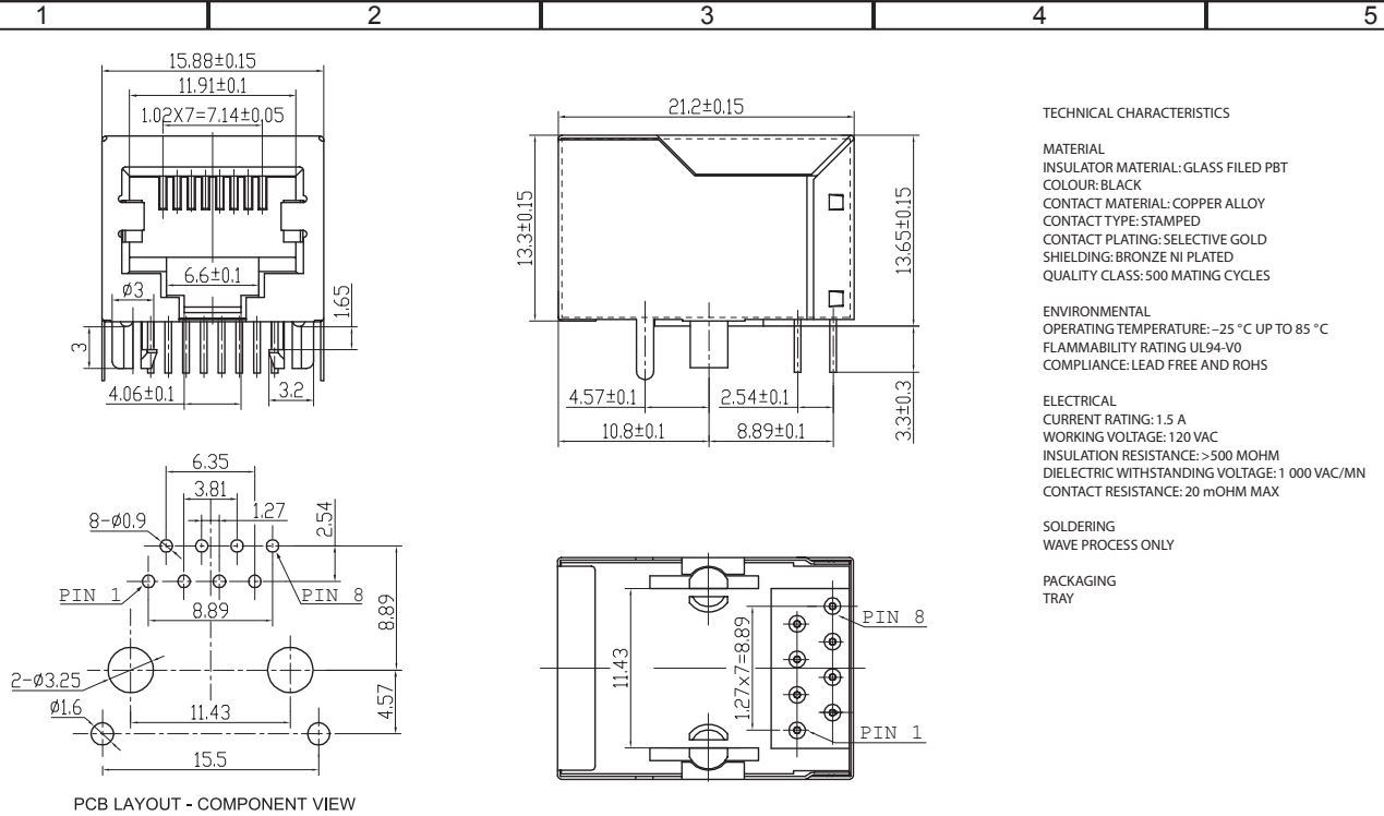
PCB LAYOUT - COMPONENT VIEW
