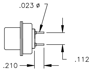
SIGNAL CONTACTS
