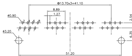
PC Board Layout Component Side Shown
