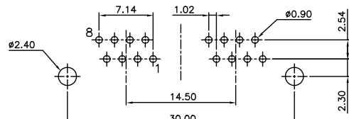
PC Board Layout Component Side Shown
