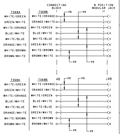
ELECTRICAL SCHEMATIC T568A OR T568B WIRING
