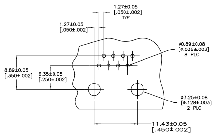
RECOMMENDED PRINTED CIRCUIT BOARD MOUNTING HOLE LAYOUT VIEW SHOWN IS COMPONENT SIDE OF BOARD
